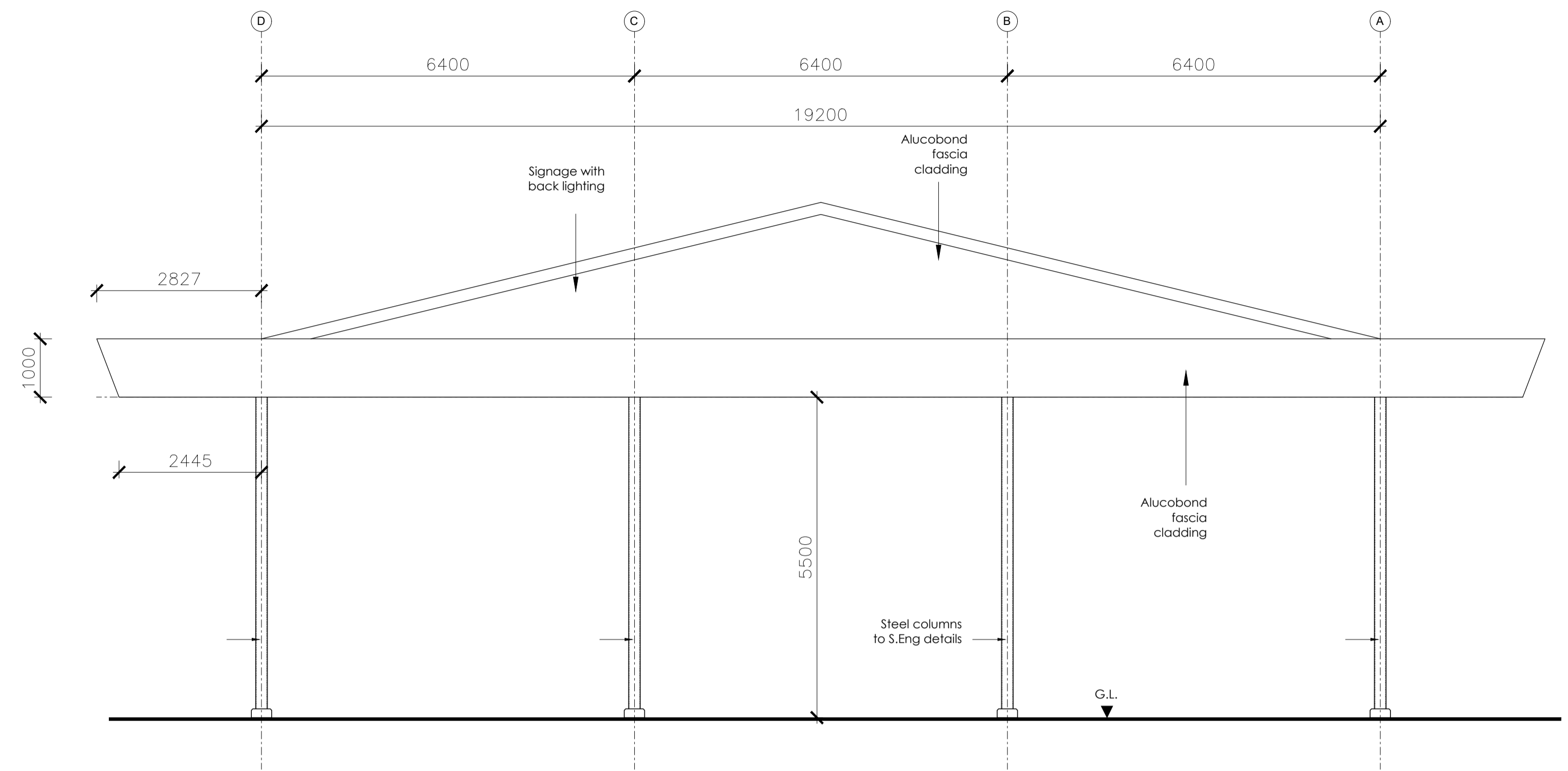
Toll Gate Canopy - Rear Elevation
