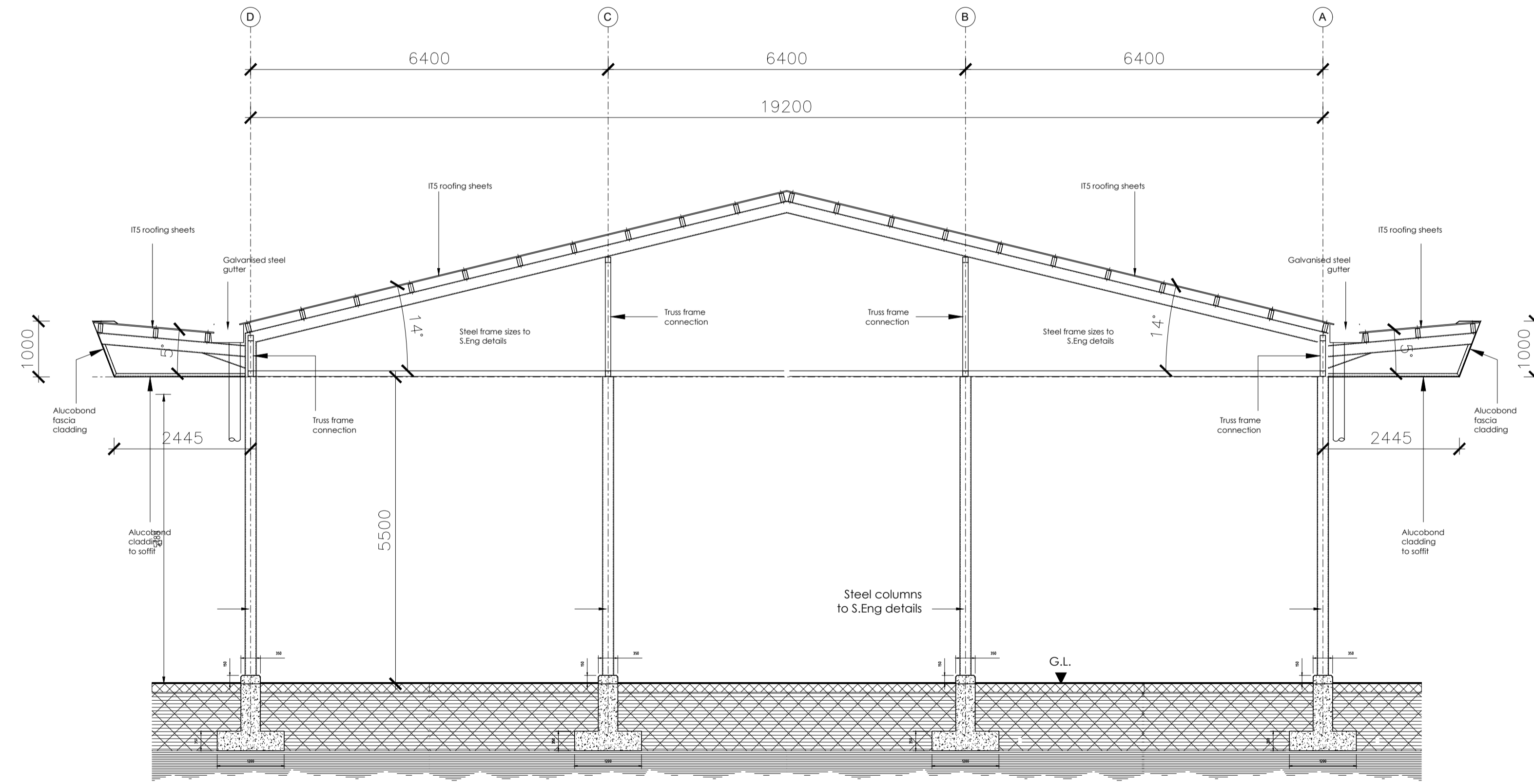
Toll Gate Canopy - Typical Section
