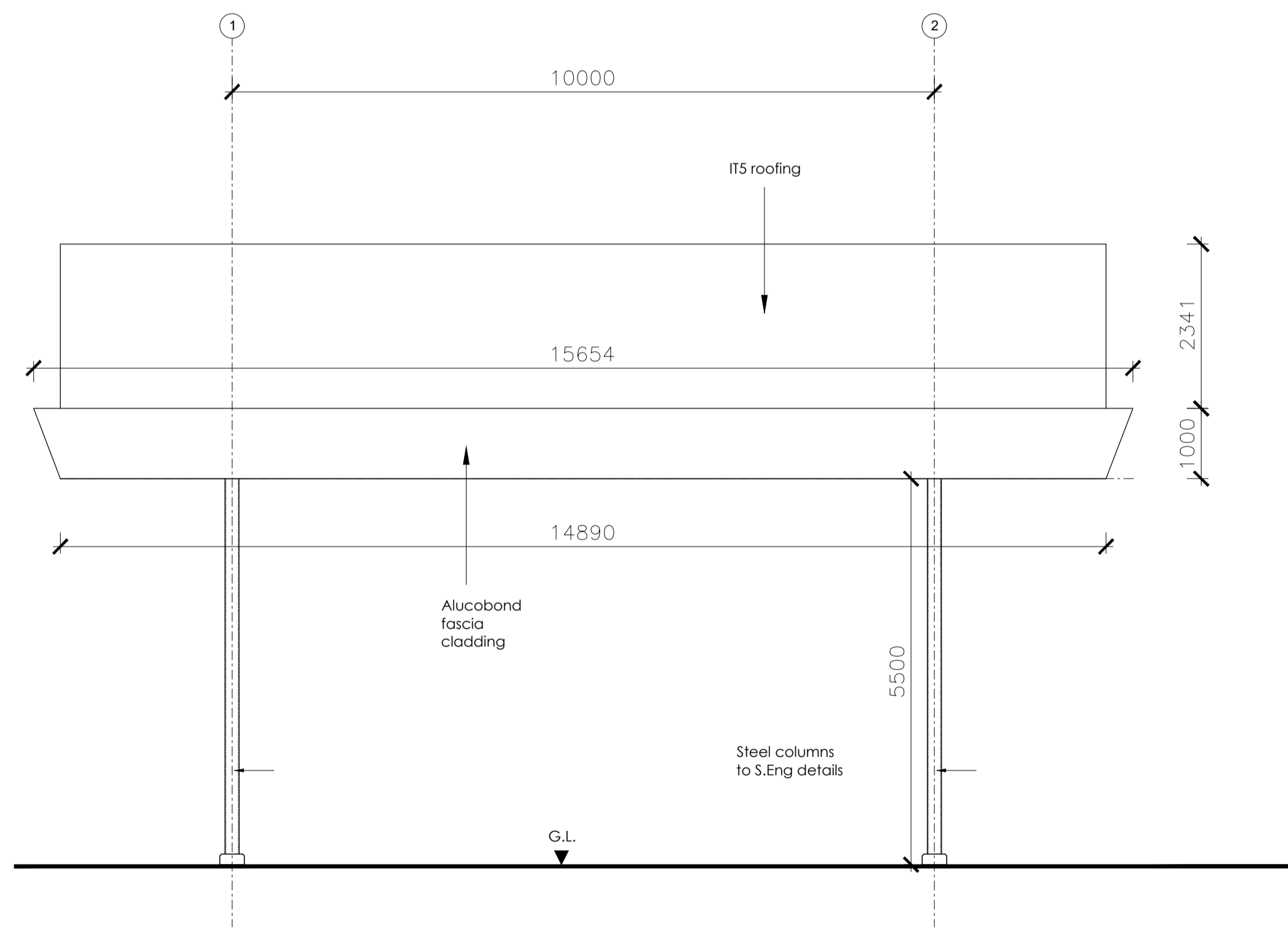
Toll Gate Canopy - Typical Side Elevation
