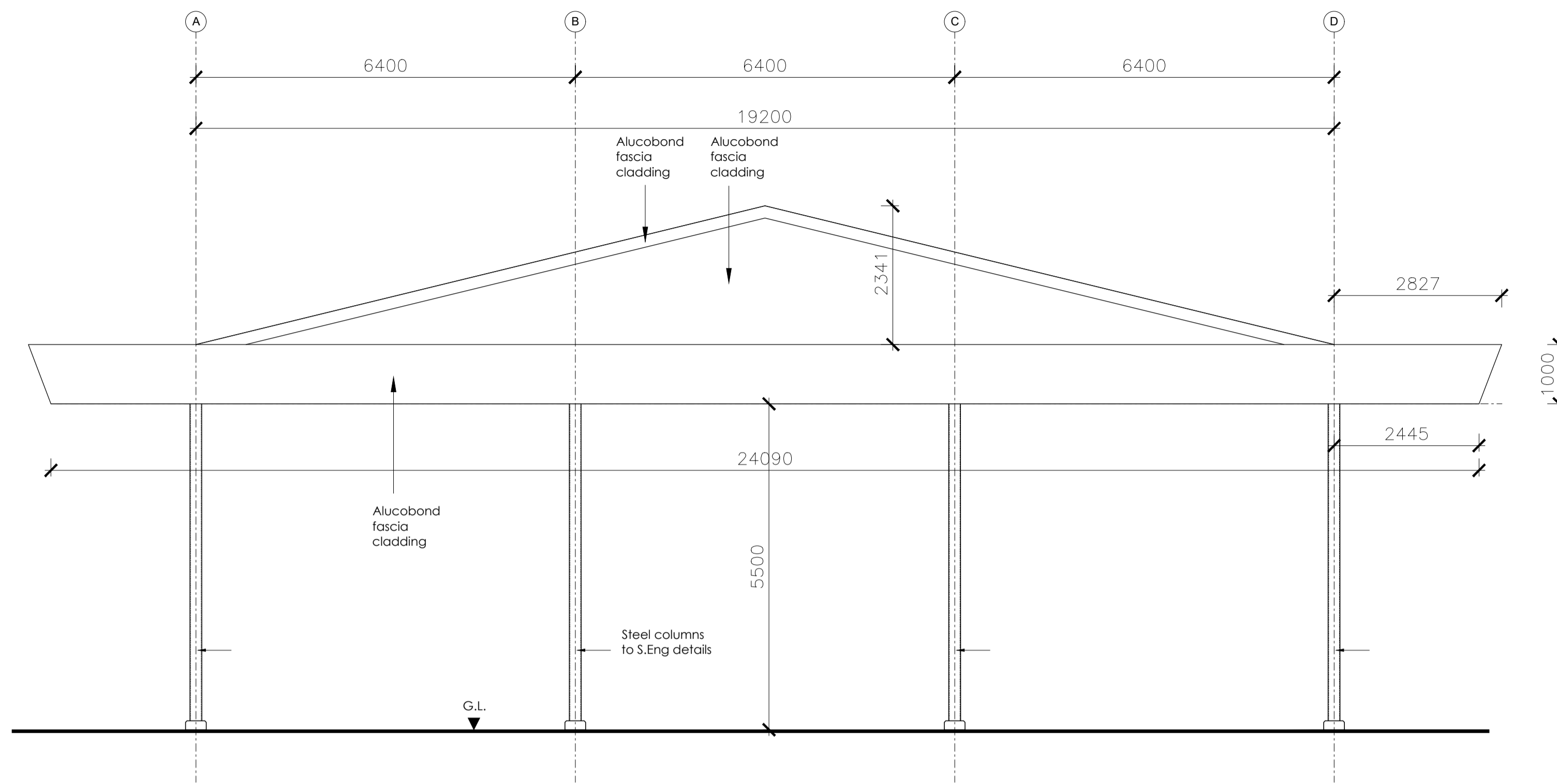
Toll Gate Canopy - Front Elevation
